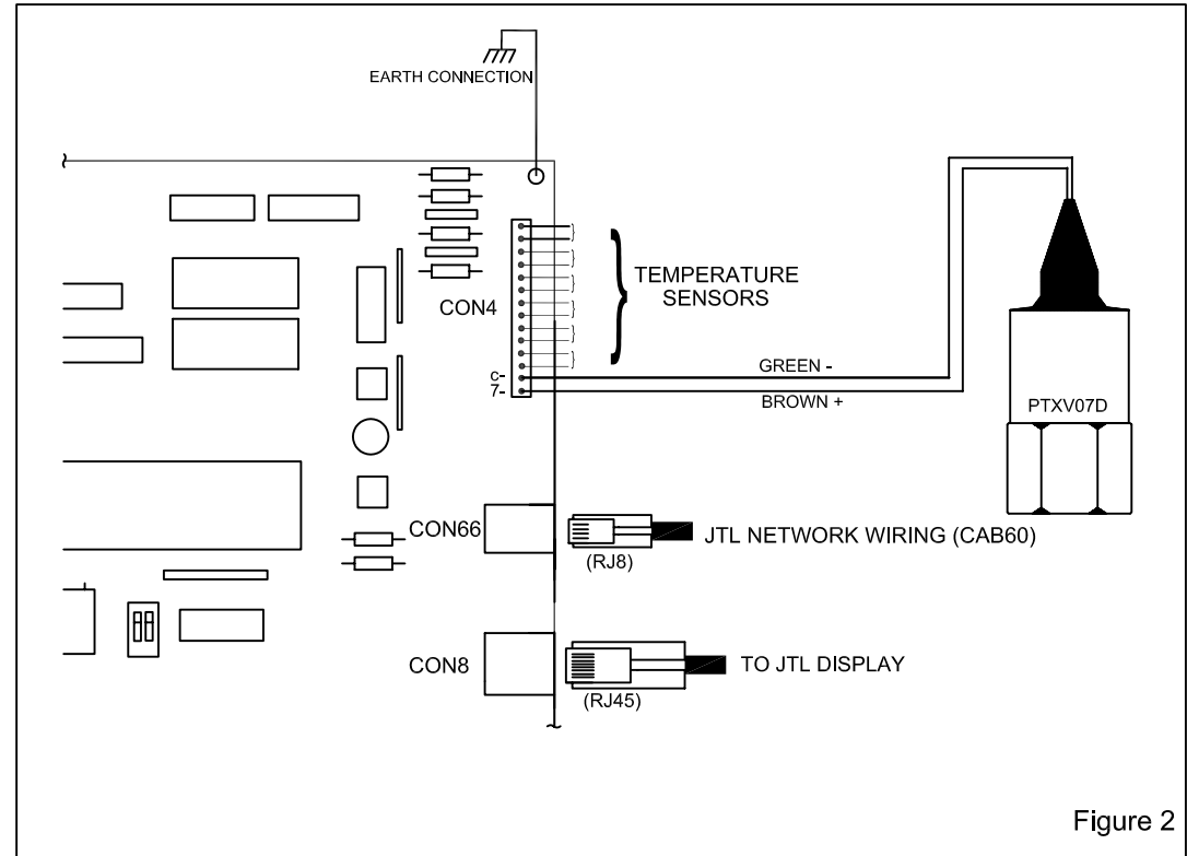
LAxx CONTROLLERS
