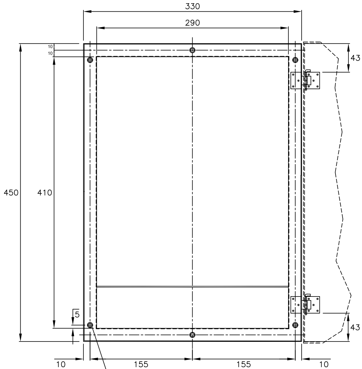
FRONT VIEW (WITH DOOR OPEN)
